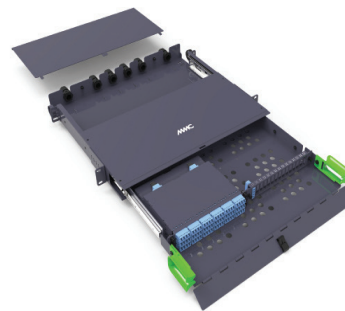
P/N: DCPANEL1U with MTP® OM3 slim cassettes & OM3 loaded LC Quad adapter plate
